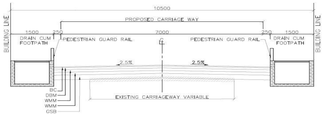
TCS - IIA TWO LANE CONCENTRIC WIDENING RECONSTRUCTION IN BUILTUP AREA WITH SIDE DRAIN CUM FOOTPATH
