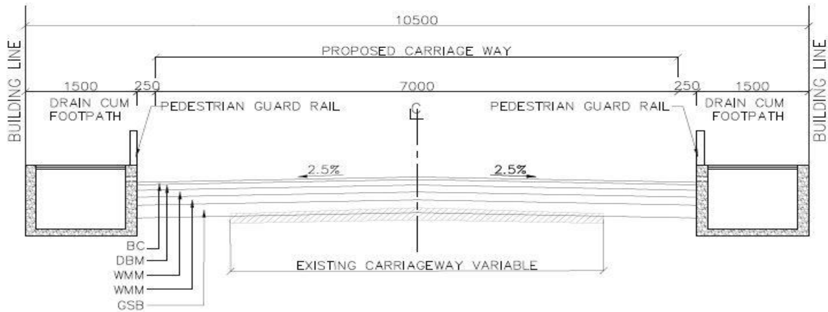
TCS - IIA TWO LANE CONCENTRIC WIDENING RECONSTRUCTION IN BUILTUP AREA WITH SIDE DRAIN CUM FOOTPATH
