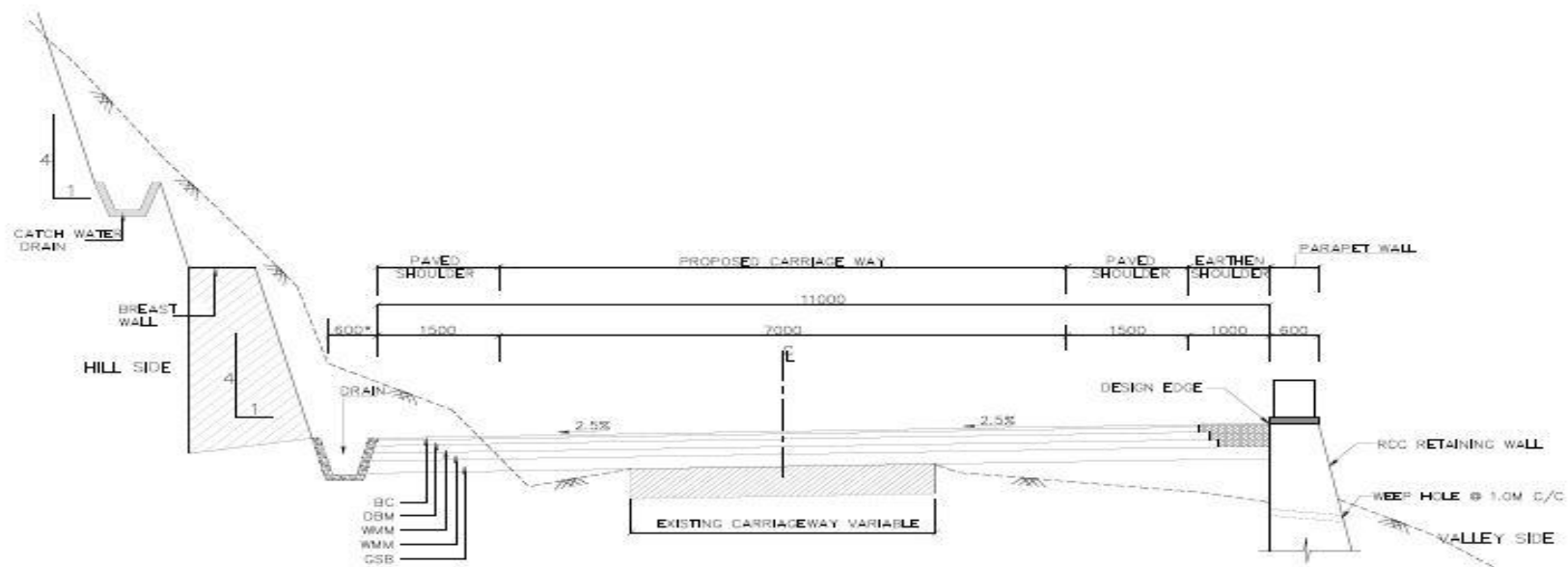
TCS - V TWO LANE NEW CONSTRUCTION AT HAIRPIN BEND
